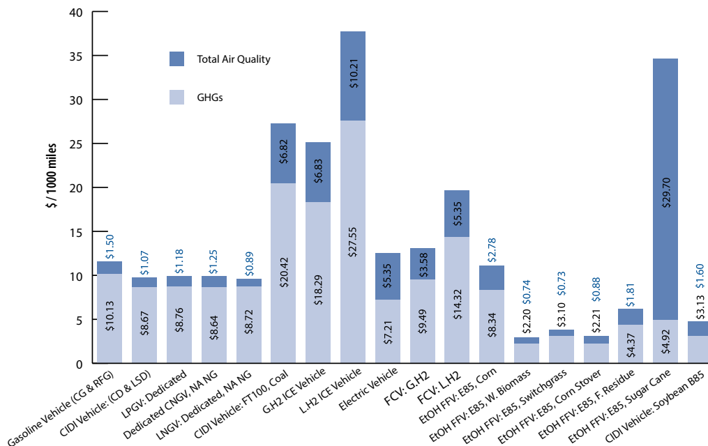
Figure 1. Valued externalities of alternative fuels (2007$/1,000 miles)
