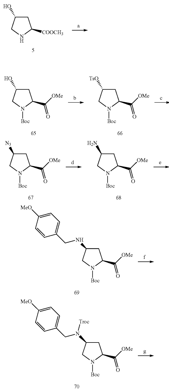
Scheme 3. Synthesis of compounds 74-88
