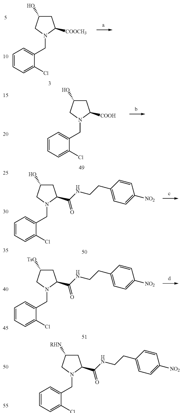
Scheme 2. Synthesis of compounds 52-64.
